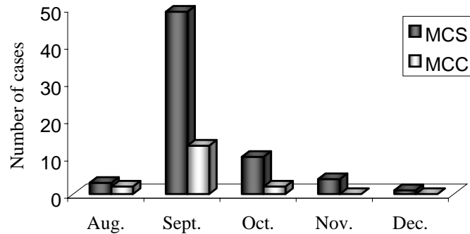
Figure 1: Time distribution of MCSs and MCCs during 1990-94
