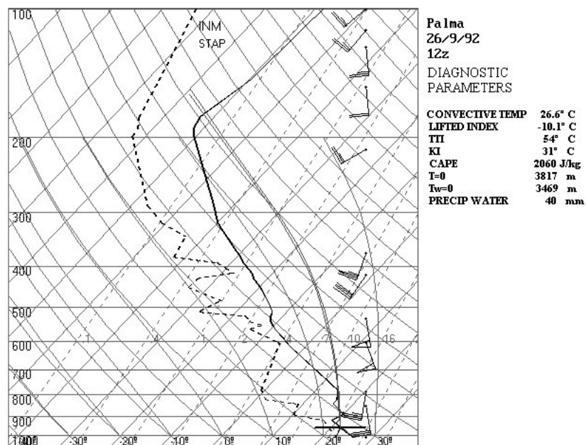
Figure 5. Skew T - Log p plot of the sounding taken from Palma de Mallorca station on 1200 UTC, 26 September 1992. Full barb is 5 \text{ m s}^{-1} .
