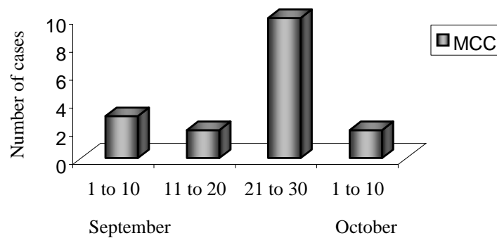
Figure 2. MCC distribution during 1990-94
