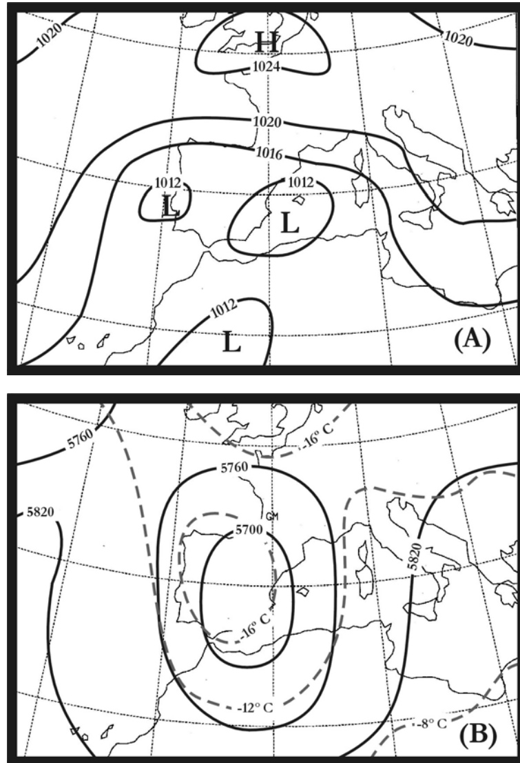
Figure 4. Same as Fig. 3 except for Class 2.
