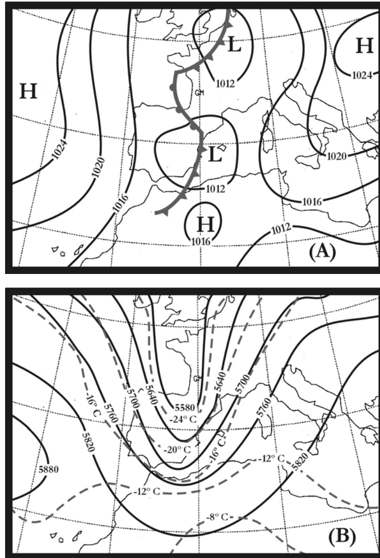
Figure 3. Schematic representation of the two categories found. Synoptic pattern scheme for Class 1. A) Surface level, B) 500 hPa level
